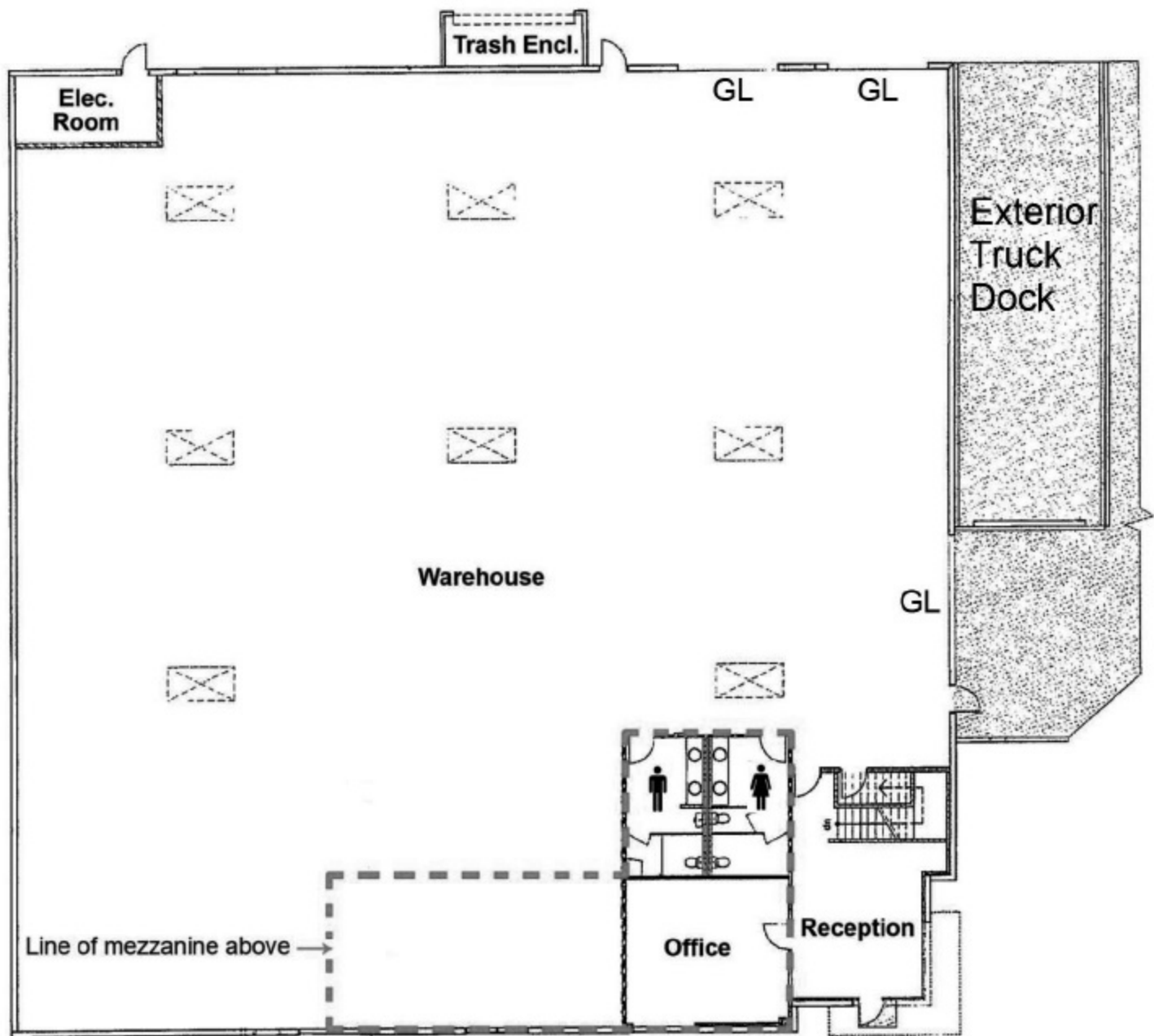
Ground Level Floor Plan
